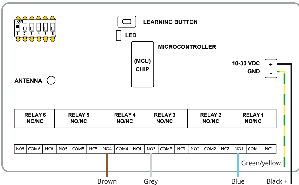
Fig.1 Connection bridge
